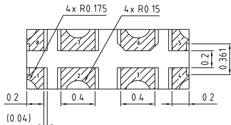
BOTTOM VIEW (view from bottom)
