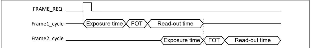
Figure 14: Internal exposure request for 2 frames with exposure time < read-out time
