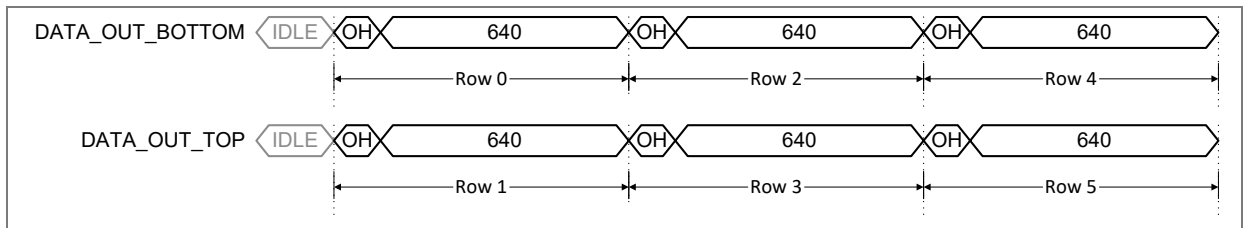
Figure 17: Data output timing with 16 channels
