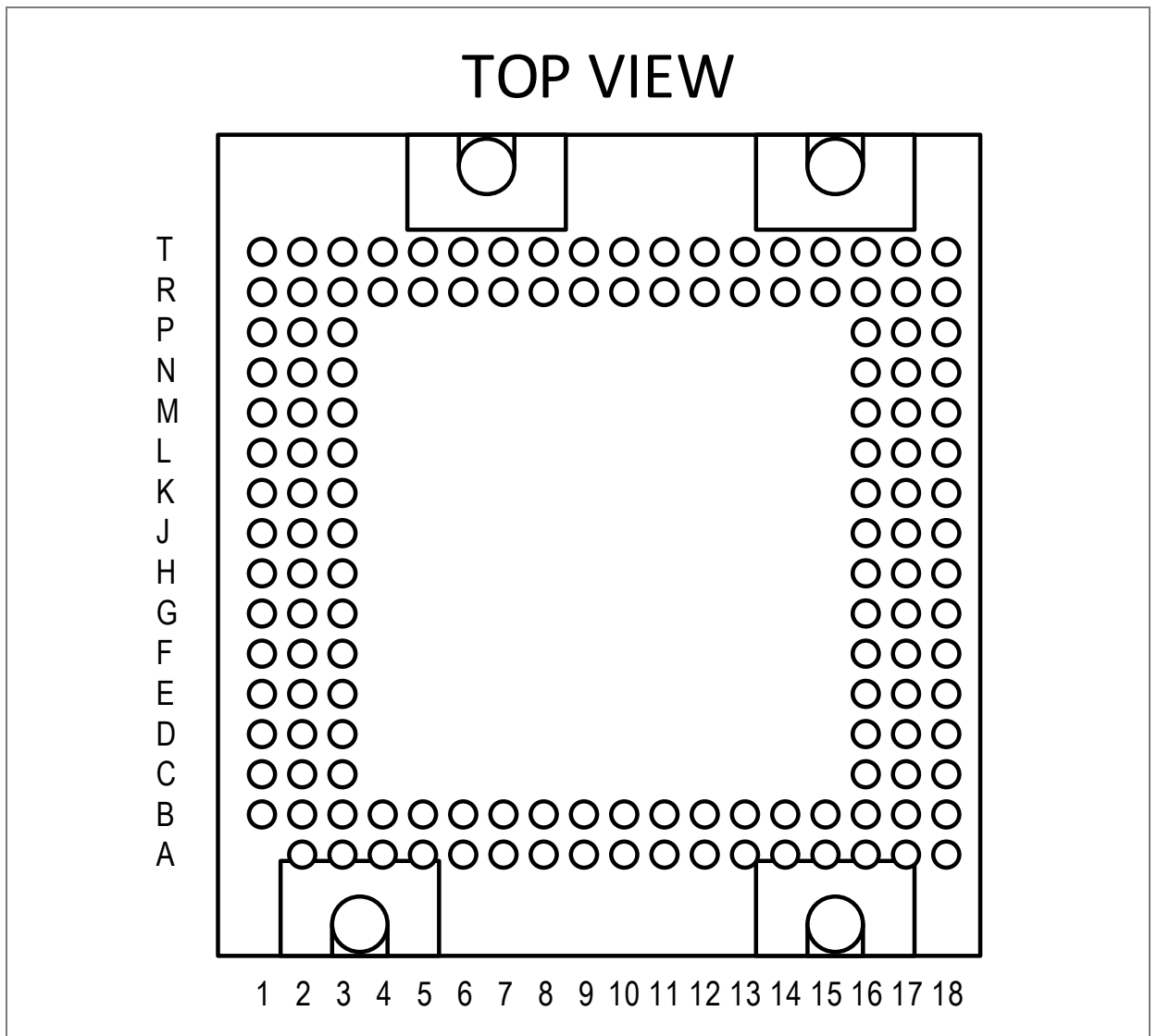
Figure 3: Pin diagram of CMV20000
