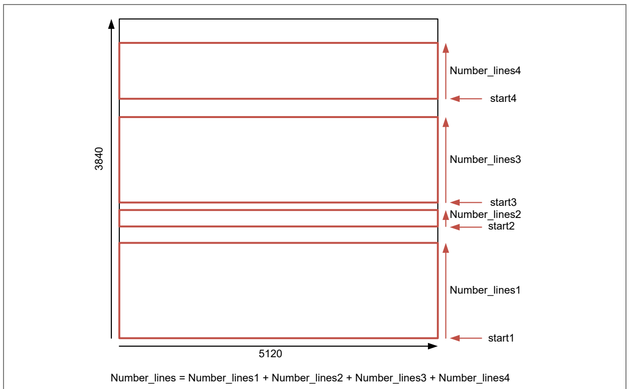
Figure 31: Example of 4 sub-windows read-out
