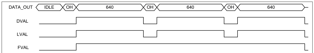
Figure 21: xVAL timing in 16 output mode
