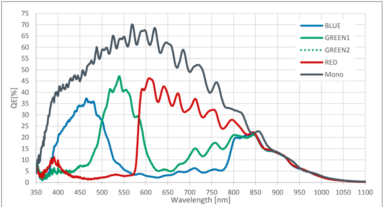
Figure 4: Quantum efficiency
