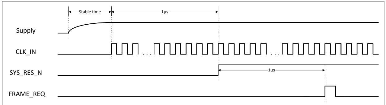
Figure 7: Startup sequence for 480 Mbps @12-bit
