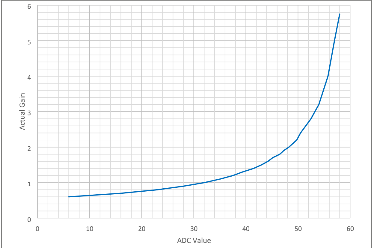
Figure 34: ADC gain vs. actual gain
