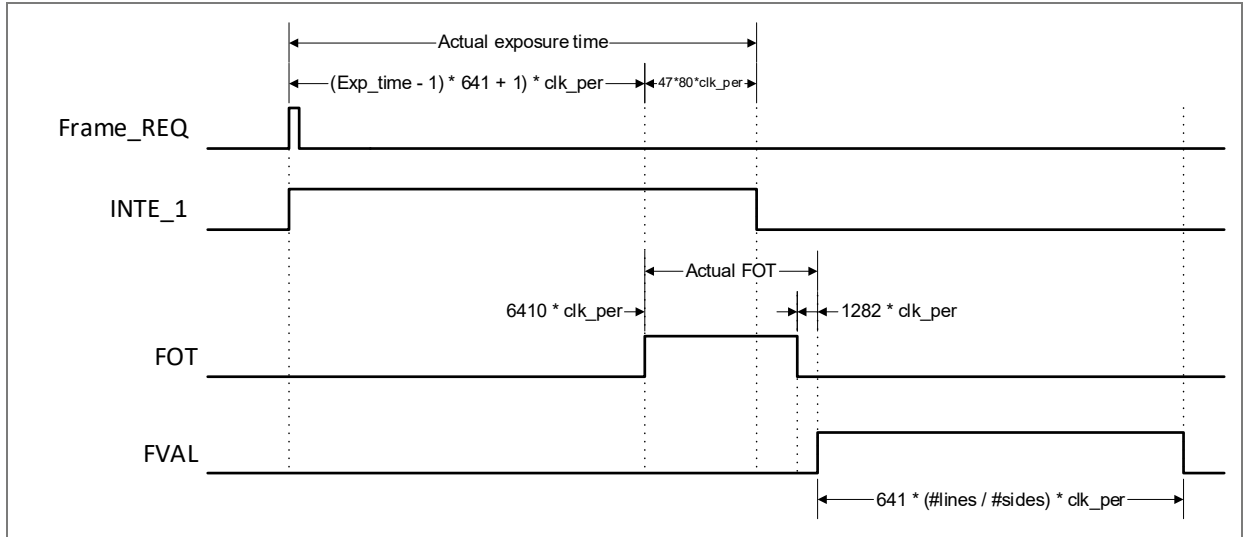
Figure 26: Frame timing
