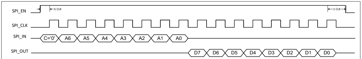
Figure 11: SPI read
