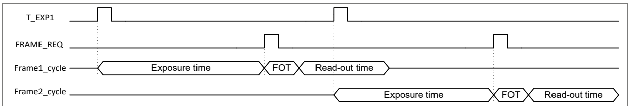
Figure 15: External exposure request for 2 frames
