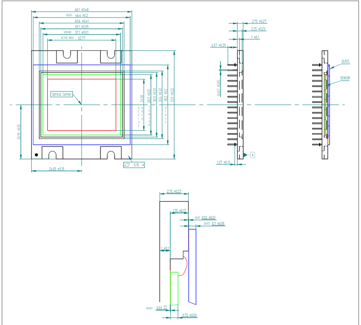
Figure 37: Assembly outline drawing
