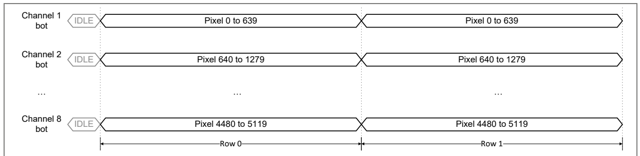
Figure 20: Pixel mapping using 8 output channels
