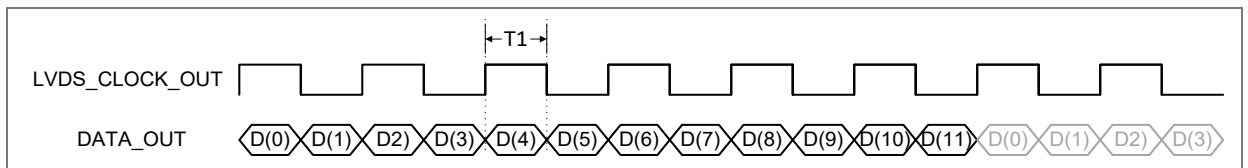
Figure 16: 12-bit pixel data on an LVDS channel
