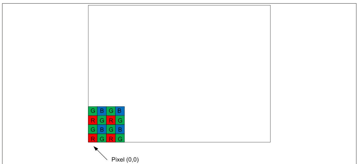
Figure 35: RGB bayer pattern order
