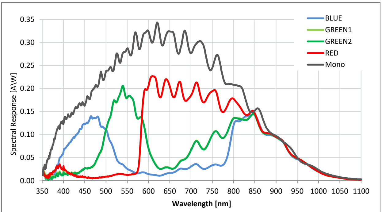
Figure 5: Spectral response
