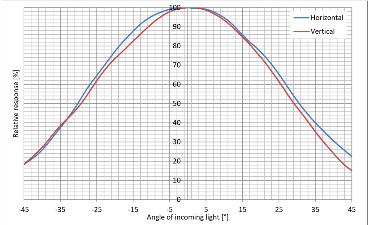
Figure 6: Angular response
