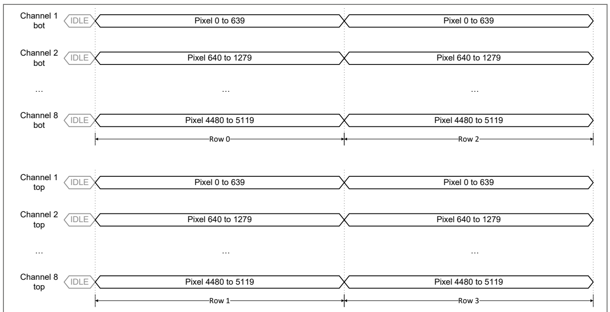
Figure 19: Pixel mapping using 16 output channels
