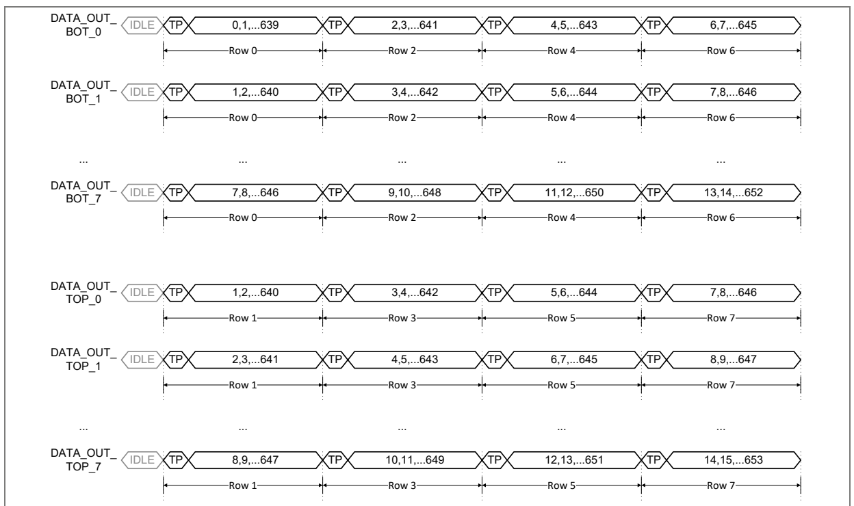
Figure 24: Test pattern data
