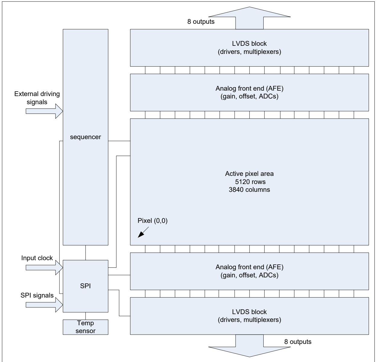
Figure 1: Functional blocks of CMV20000
