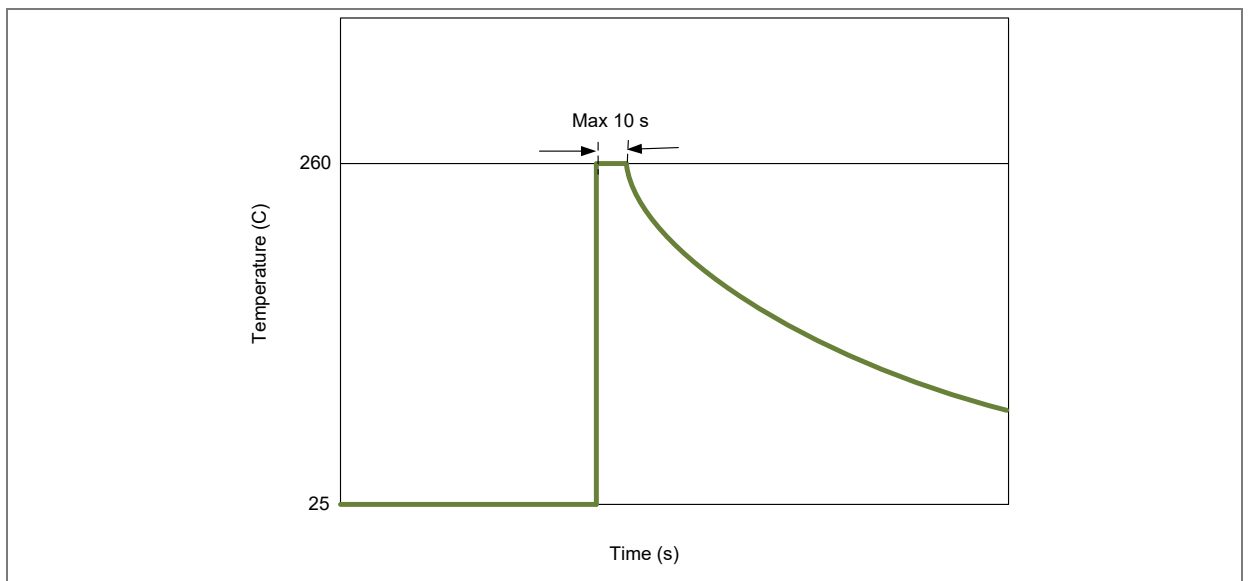
Figure 38: Wave soldering profile
