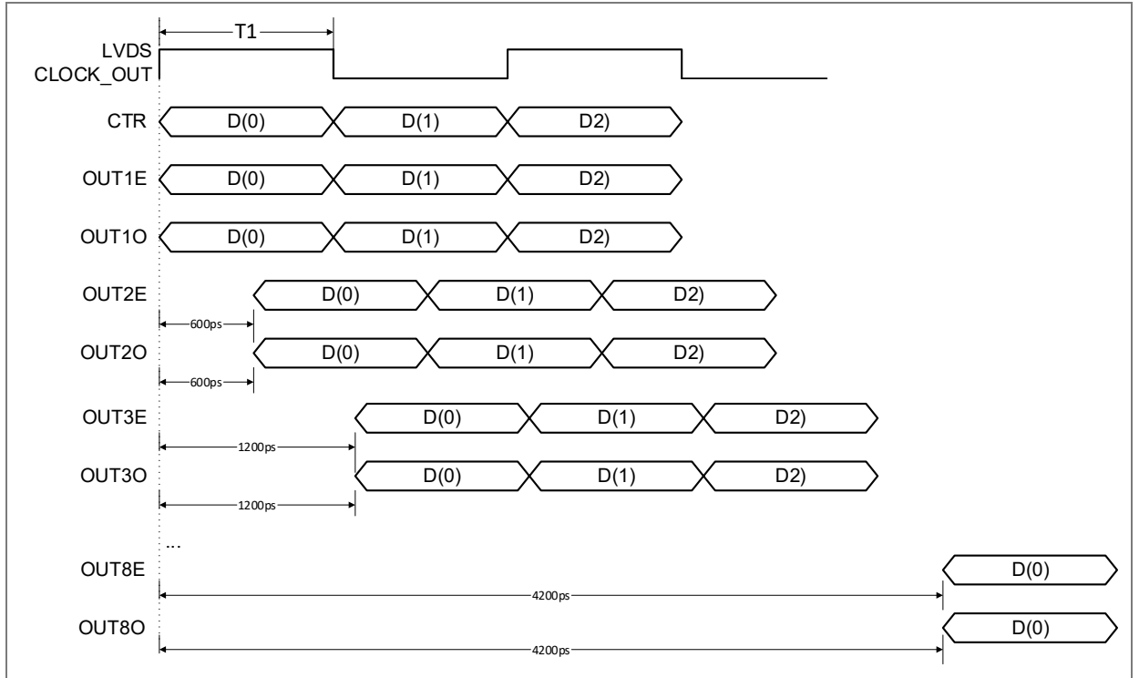
Figure 23: LVDS output skew
