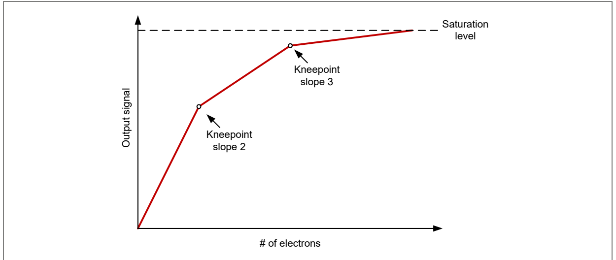
Figure 28: Piecewise linear response
