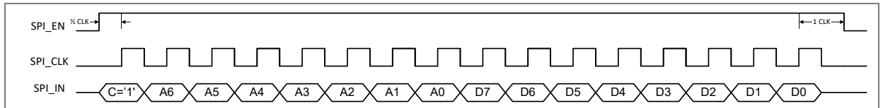
Figure 9: SPI write
