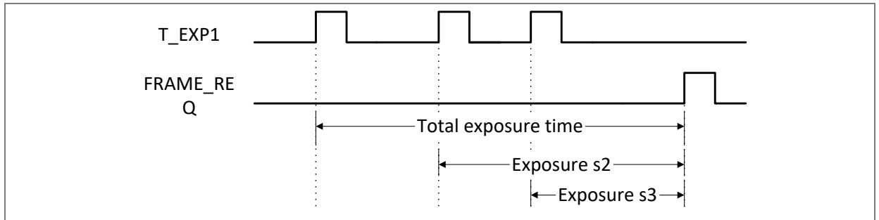
Figure 29: PLR with external exposure mode
