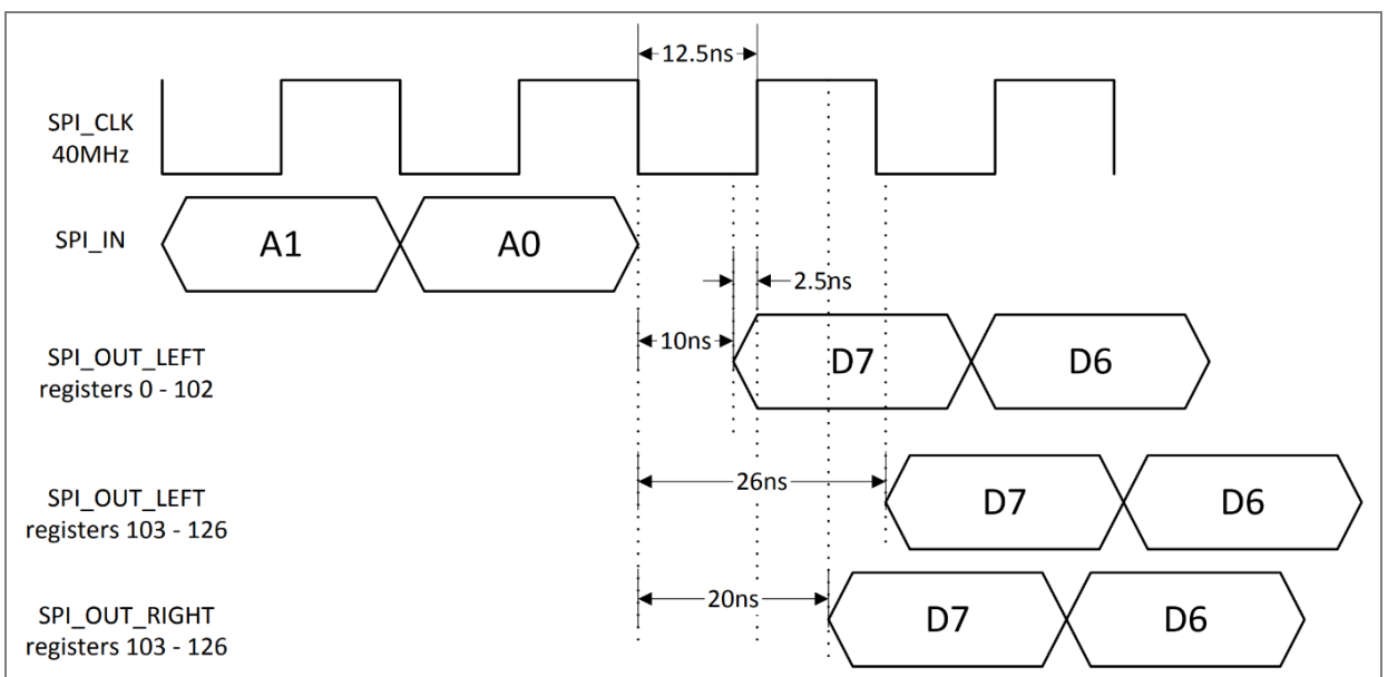
Figure 12: SPI delay
