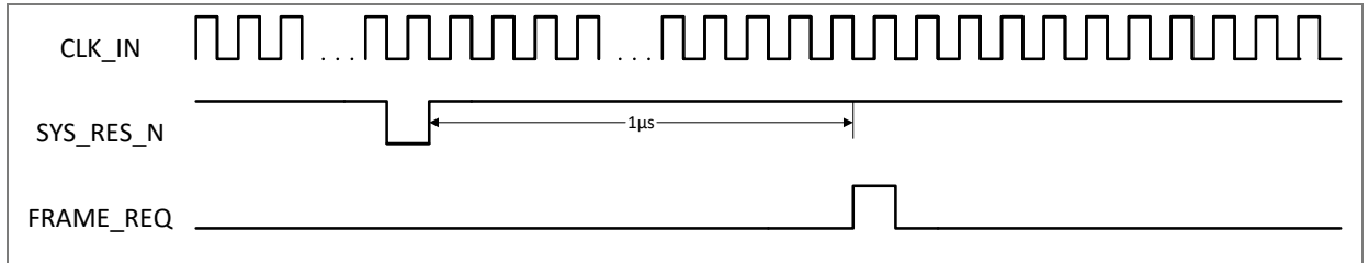
Figure 8: Reset sequence
