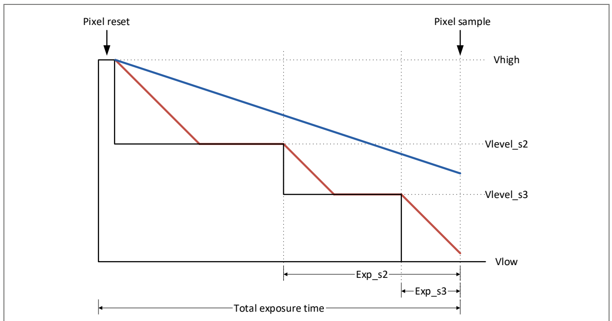
Figure 27: Piecewise linear response details
