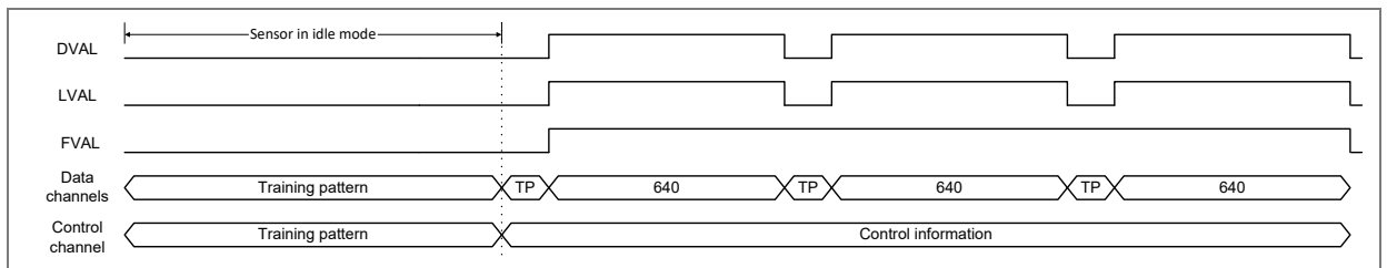
Figure 22: Training pattern timing
