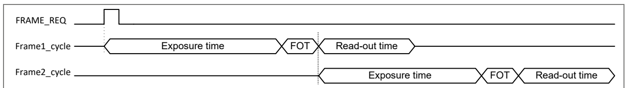
Figure 13: Internal exposure request for 2 frames
