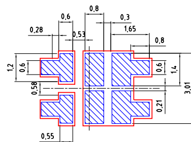
solder stencil
