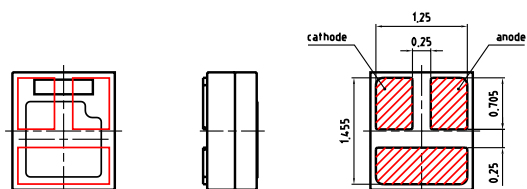
Component Location on Pad
