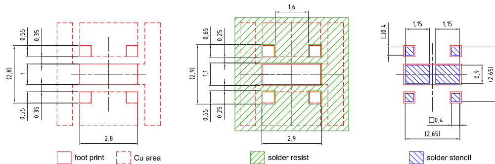
Alternative Solder pad design for pedestal MCPB
