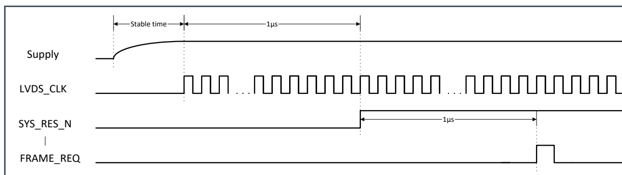
Figure 12: Startup Sequence
