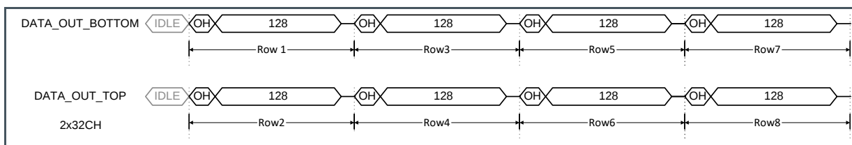
Figure 27: Data Output Timing with 64 ( 2 \times 32 ) Channels
