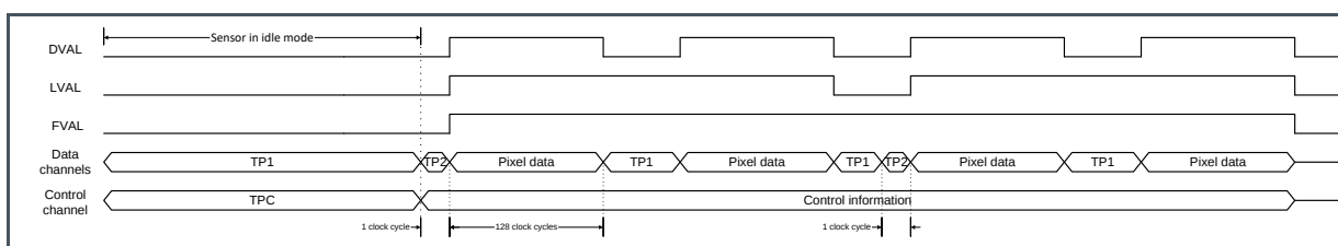
Figure 37: TP Timing
