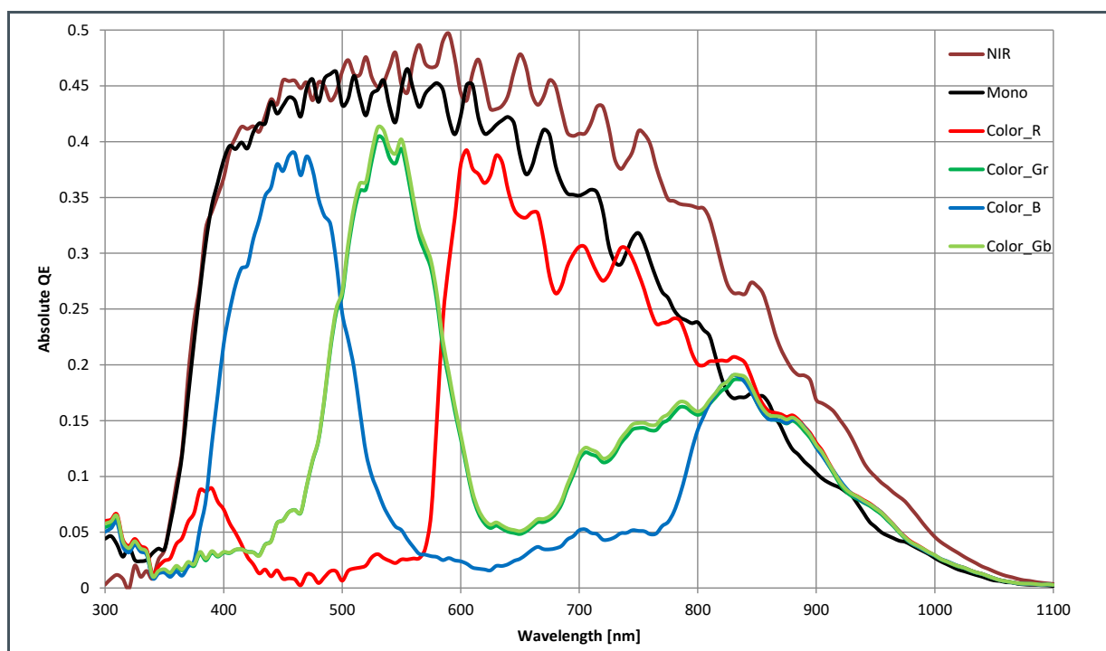
Figure 8: Quantum Efficiency
