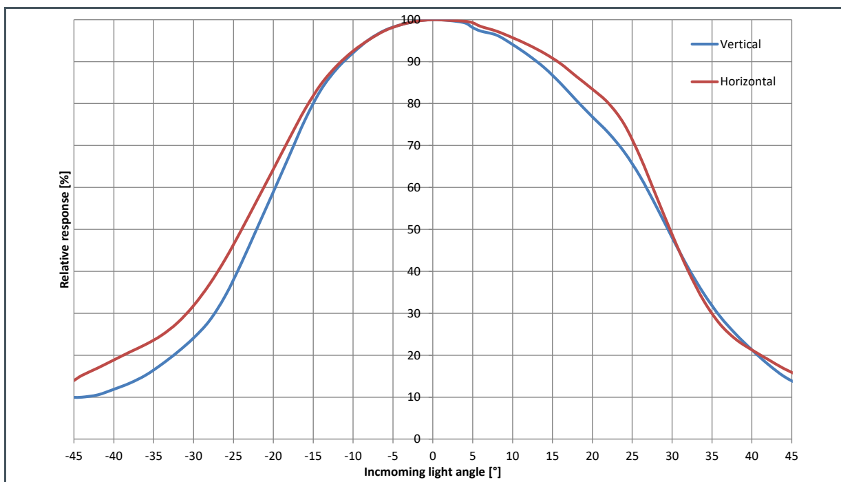
Figure 10: Angular Response
