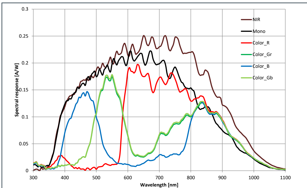
Figure 9: Spectral Response
