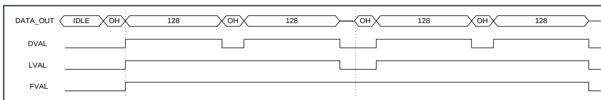
Figure 36: xVAL Timing in 2 × 16 Channel Readout Mode
