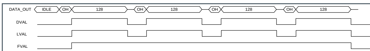
Figure 35: xVAL Timing in 2 × 32 Channel Readout Mode
