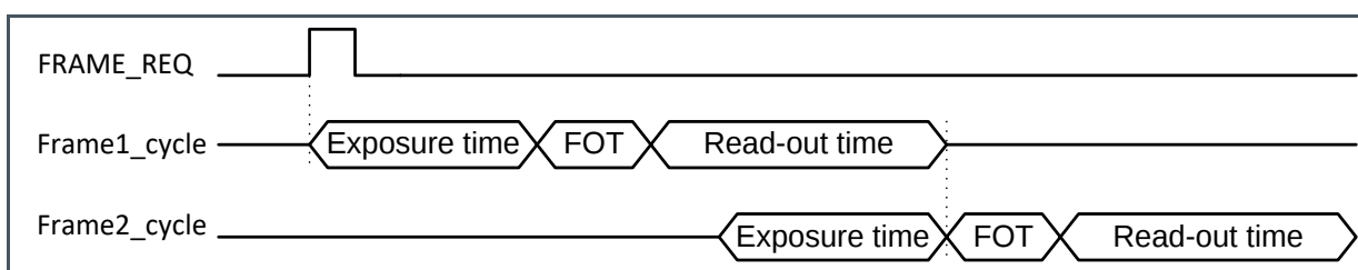
Figure 19: Internal Exposure Request for Two Frames with Short Exposure Time
