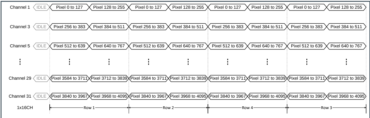
Figure 33: Pixel Mapping Using 1 × 16 Channels
