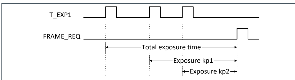
Figure 51: Multiple Slope HDR with External Exposure
