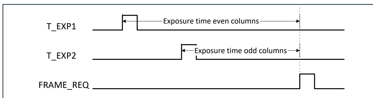
Figure 46: Interleaved HDR with External Exposure
