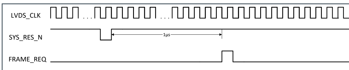
Figure 13: Reset Sequence
