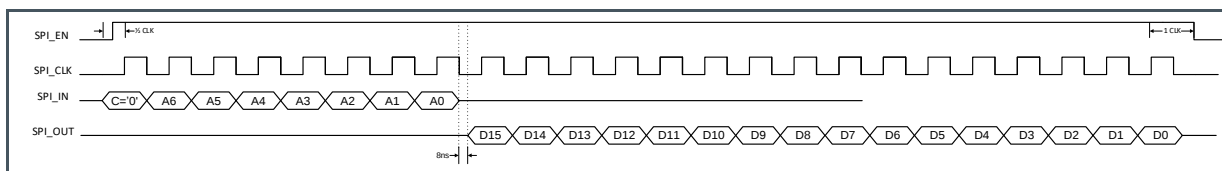
Figure 17: SPI Read
