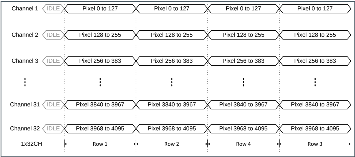
Figure 32: Pixel Mapping Using 1 × 32 Channels
