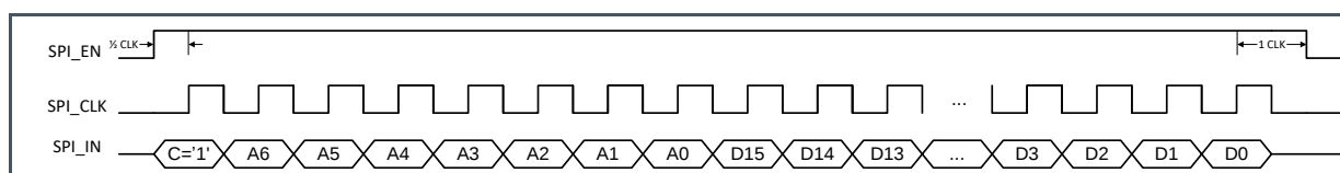
Figure 15: SPI Write
