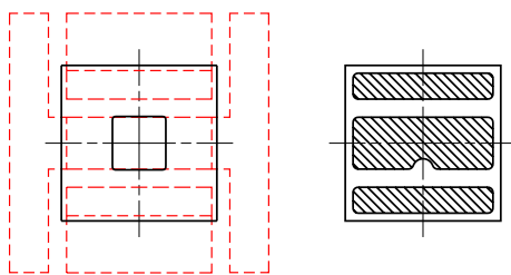
Component Location on Pad
