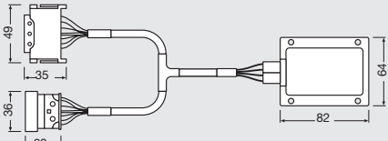
LEDDriving® SMART CANBUS (Acc, per H7-LED) LEDSC03-2HFB
