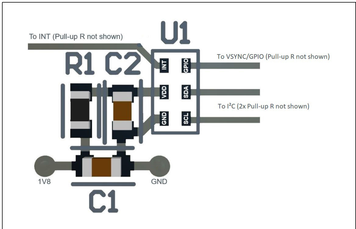
Figure 93: TCS3410 Recommended Part Placement
