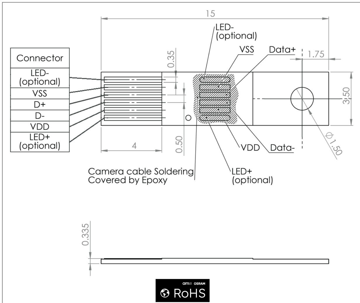
Figure 21: FlexPCB connector outline drawing (1)(2)(3)(4)
