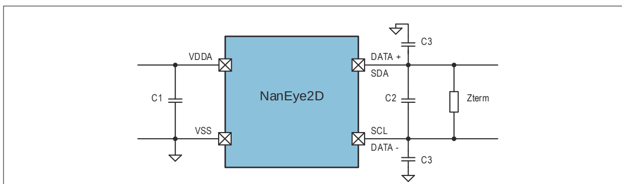
Figure 17: External components LVDS
