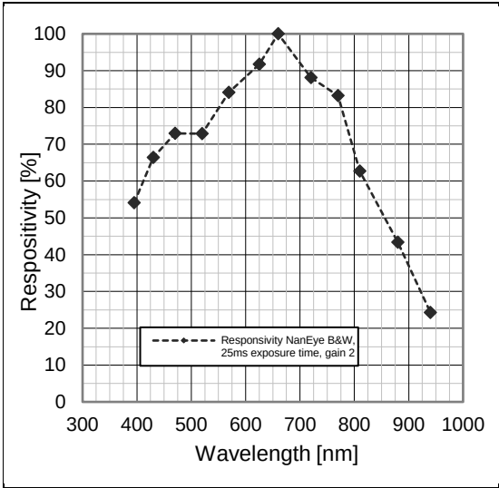
Figure 1: B&W spectral response
