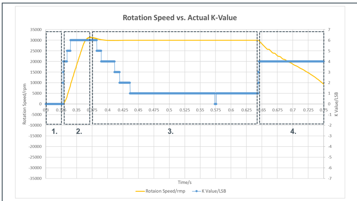
Figure 11 : Exemplary Acceleration Profile - Zoom in Section
