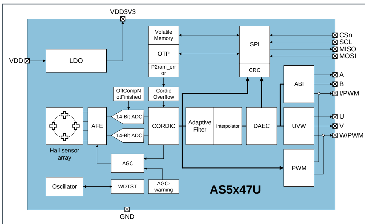
Figure 1: Block Diagram AS5x47U
